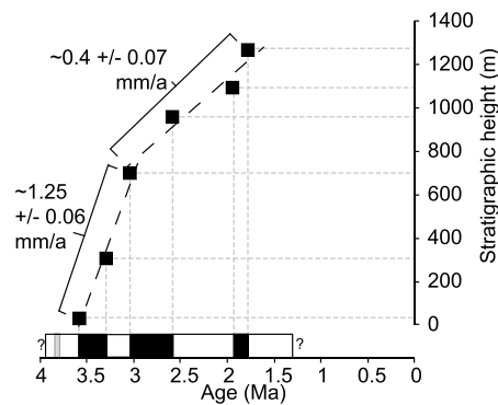
Figure 8. Sediment-accumulation rates within the Beiertuokuoyi piggyback basin. Stratigraphic height refers to the measured height within the magnetostratigraphic section.
