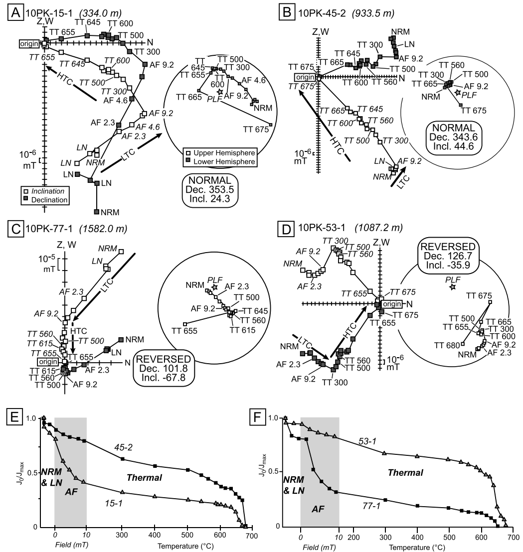
Figure 5. (a–d) Representative examples of paleomagnetic results using stepwise alternating field and thermal demagnetization of selected oriented samples. Zijderveld and equal area plots are shown, with some of the steps labeled. Most samples displayed multiple temperature components, and examples of the low-temperature component (LTC) and high-temperature component (HTC) are of the ChRM are shown. (e, f) Plots showing the decay of the magnetic moment for the same samples in Figures 5a–5d. NRM = natural remanent magnetization, LN = low-temperature step (when samples were cooled in liquid nitrogen), and AF = alternating field (in mT). Both magnetite and hematite are interpreted as ChRM carriers, noted by the decrease in magnetic moment between 500° and 580°C and between 660° and 680°C.
