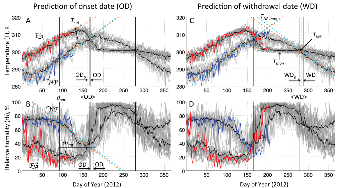
Figure 3. Prediction of onset date (OD) and withdrawal date (WD): case study 2012. (a, b) Prediction of the onset date (OD); (c, d) withdrawal date (WD) of monsoon in the EG. Air temperature at 1000 hPa (Figures 1a and 1c); relative humidity at 1000 hPa (Figures 1b and 1d). Time series from reference points (NCEP/NCAR data): previous 14 year mean (black) and 2012 values for NP (blue) and the EG (red). Grey lines show time series from the NP and EG for the training period of previous 14 years. Saturation temperature T_{sat} (Figure 1a) and saturation humidity rh_{sat} (Figure 1c) are marked by horizontal black solid lines ( T_{sat} = T_{onset} , T_{onset} and rh_{sat} calculated as intersection of mean time series for the training period from the EG and NP) and day of the saturation ( d_{sat} ) (when temperature in the EG in 2012 reaches T_{sat} )—with dark blue. Orange lines indicate trends to the mean time series in the NP and EG for the training period, light blue—trends for 2012. Black solid lines indicate mean values of the OD ( \langle OD \rangle ) and WD ( \langle WD \rangle ) for the training period. Dotted grey lines correspond to the predicted onset ( OD_p ) and withdrawal dates ( WD_p ), while solid grey lines—to actual onset and withdrawal dates for 2012.
